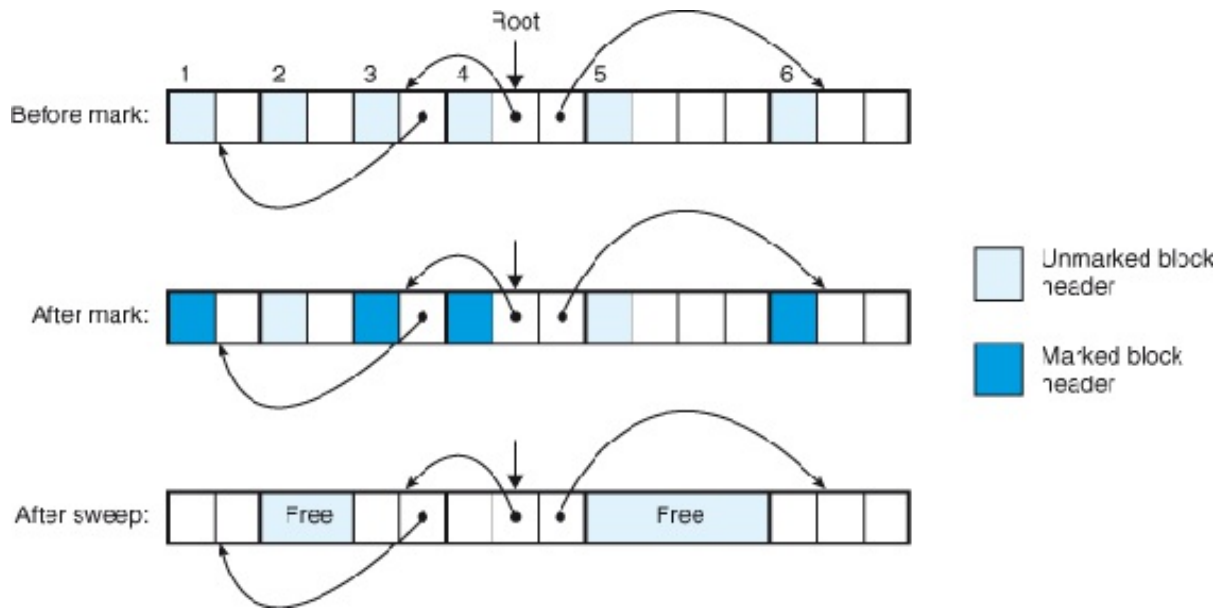
Figure 9.52 Mark&Sweep example.
