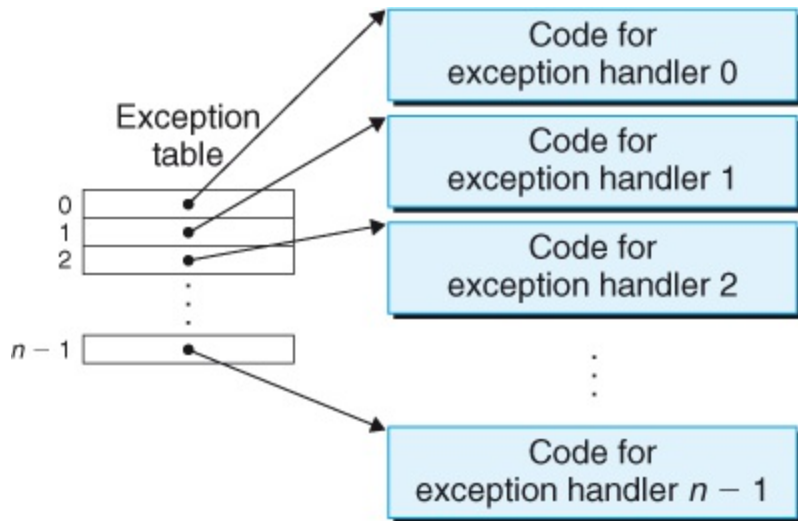
Figure 8.2 Exception table.
