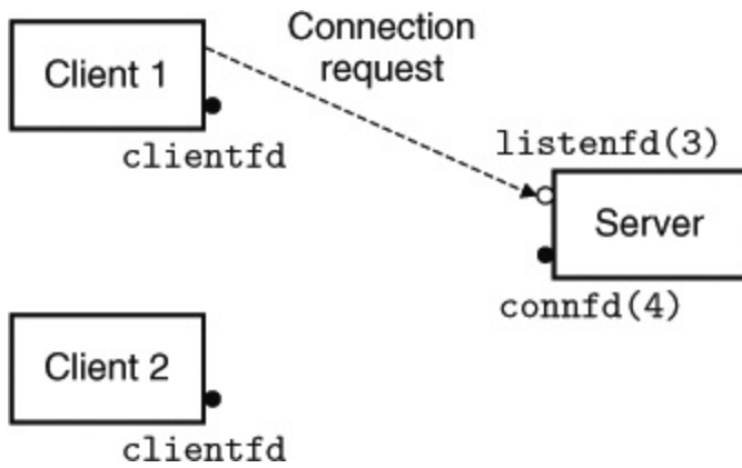
Figure 12.1 Step 1: Server accepts connection request from client.
