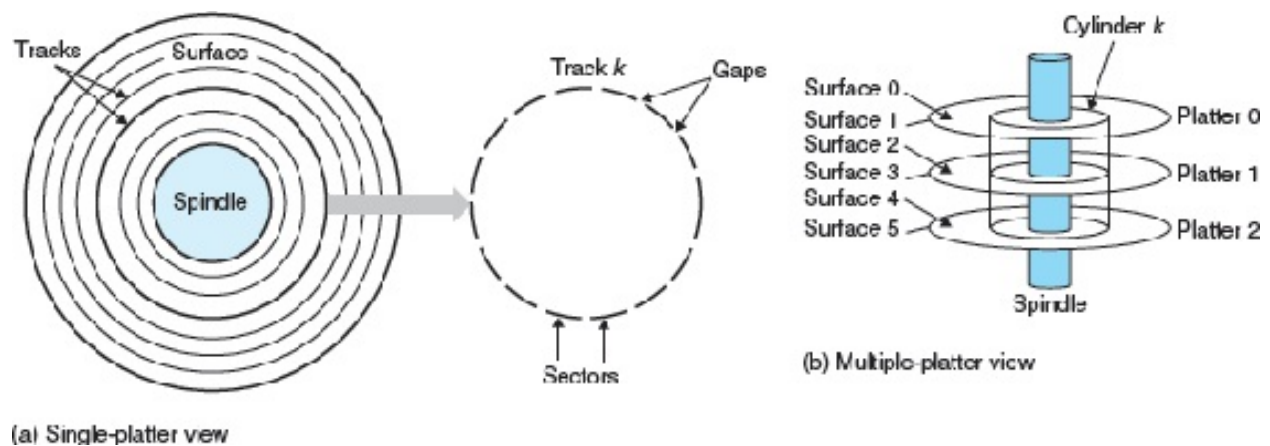
Figure 6.9 Disk geometry.
