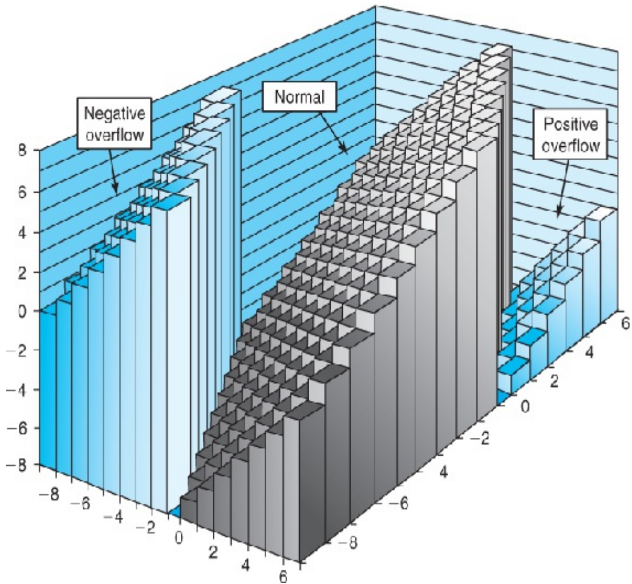
Figure 2.26 Two's-complement addition.
