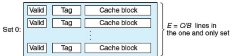
Figure 6.35 Fully associative cache ( E = C/B ).
