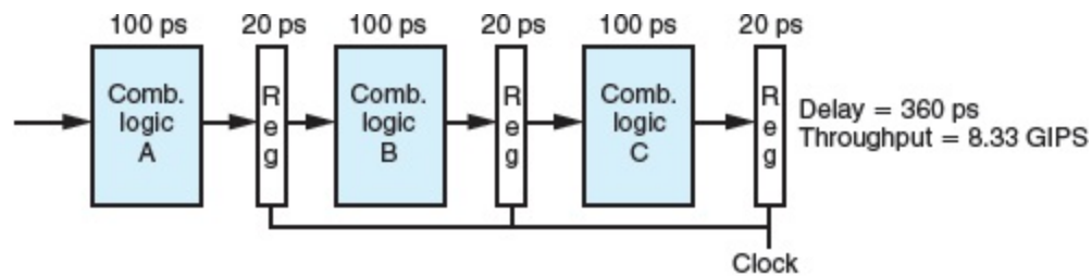
(a) Hardware: Three-stage pipeline
