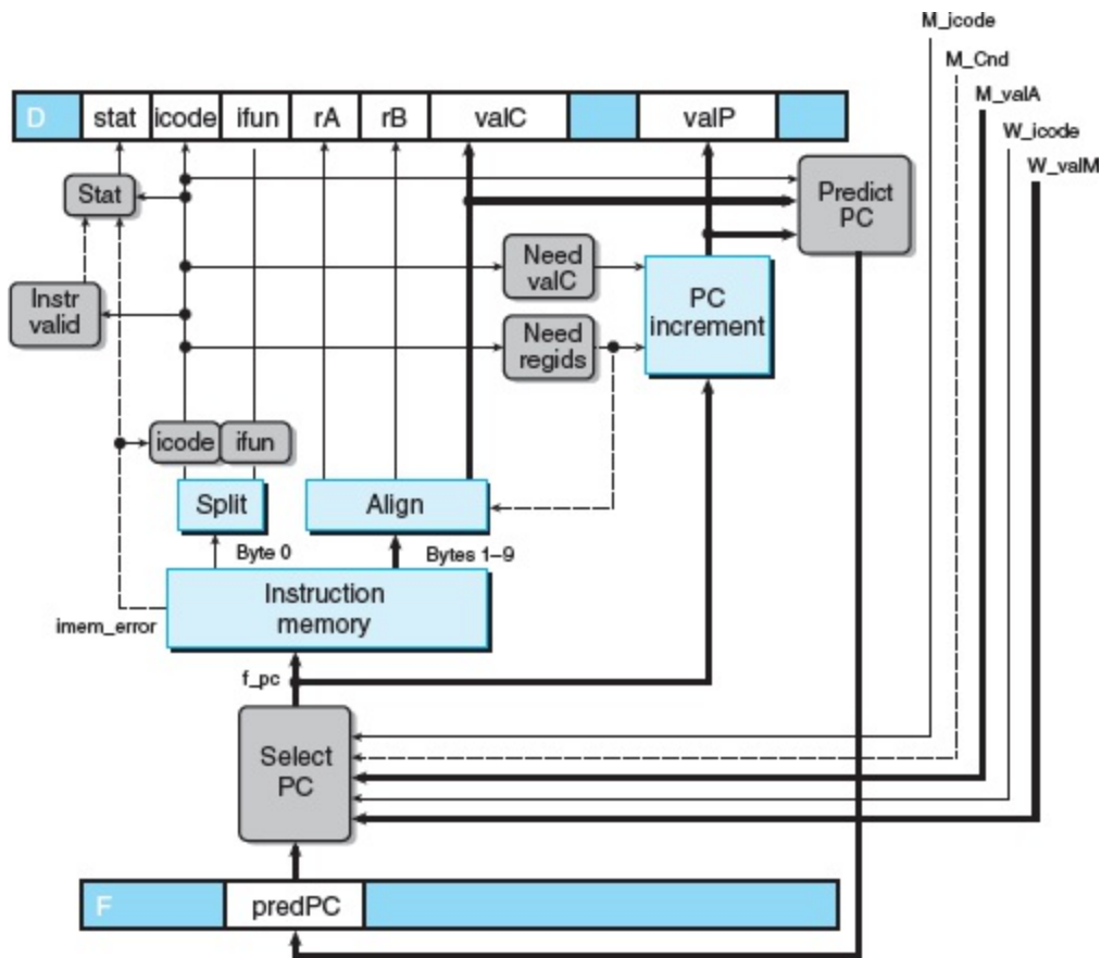
Figure 4.57 PIPE PC selection and fetch logic.
