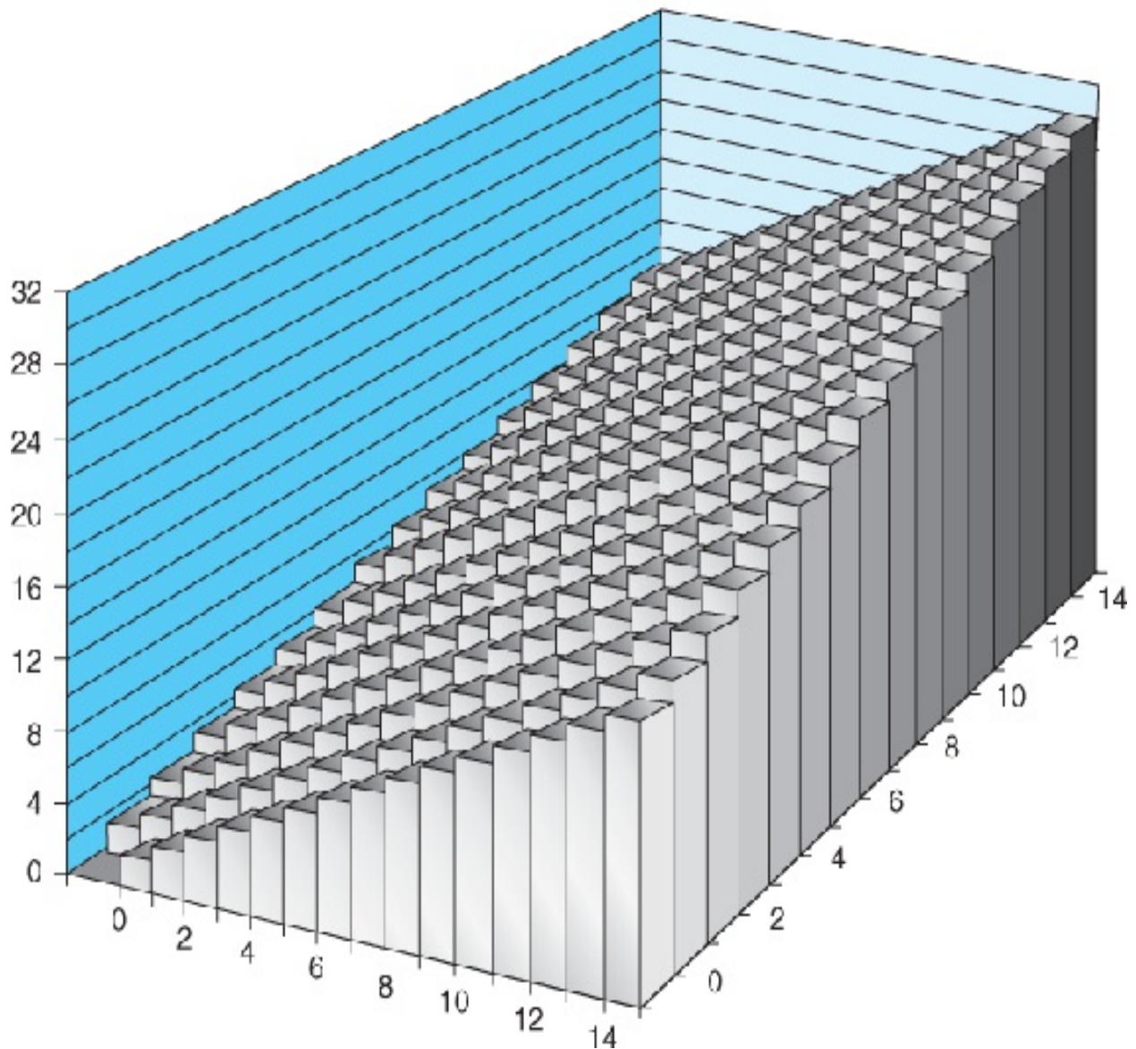
Figure 2.21 Integer addition.
