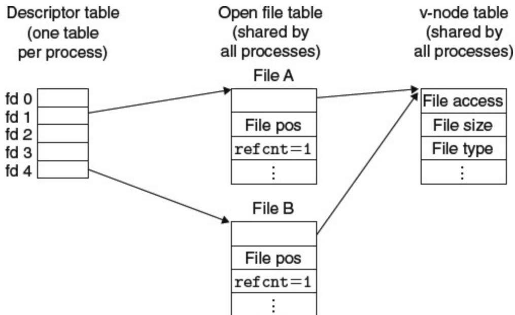
Figure 10.13 File sharing.
