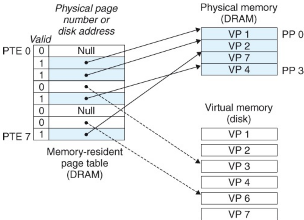
Figure 9.4 Page table.
