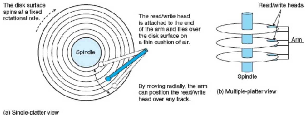
Figure 6.10 Disk dynamics.
