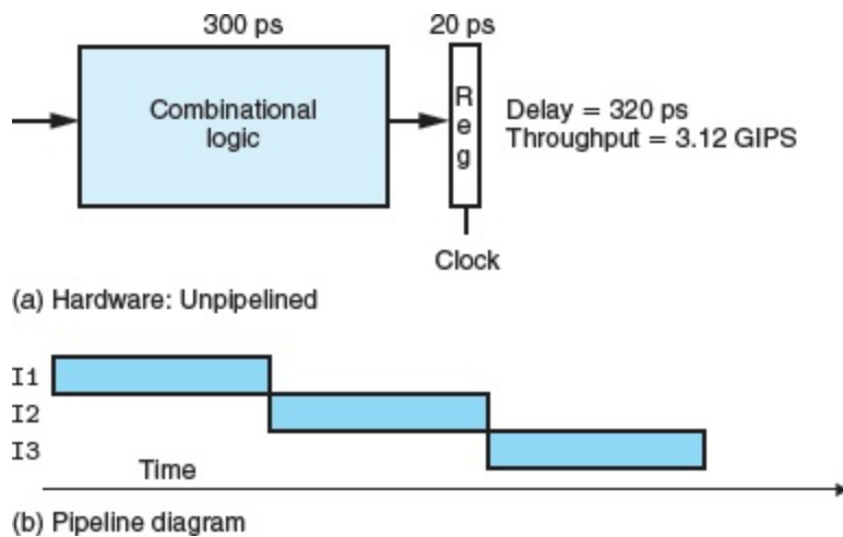
Figure 4.32 Unpipelined computation hardware.
