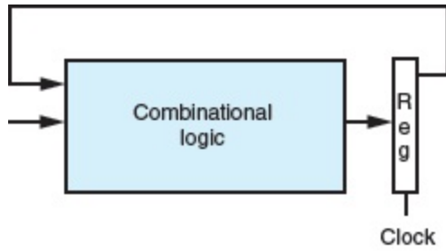
(a) Hardware: Unpipelined with feedback
