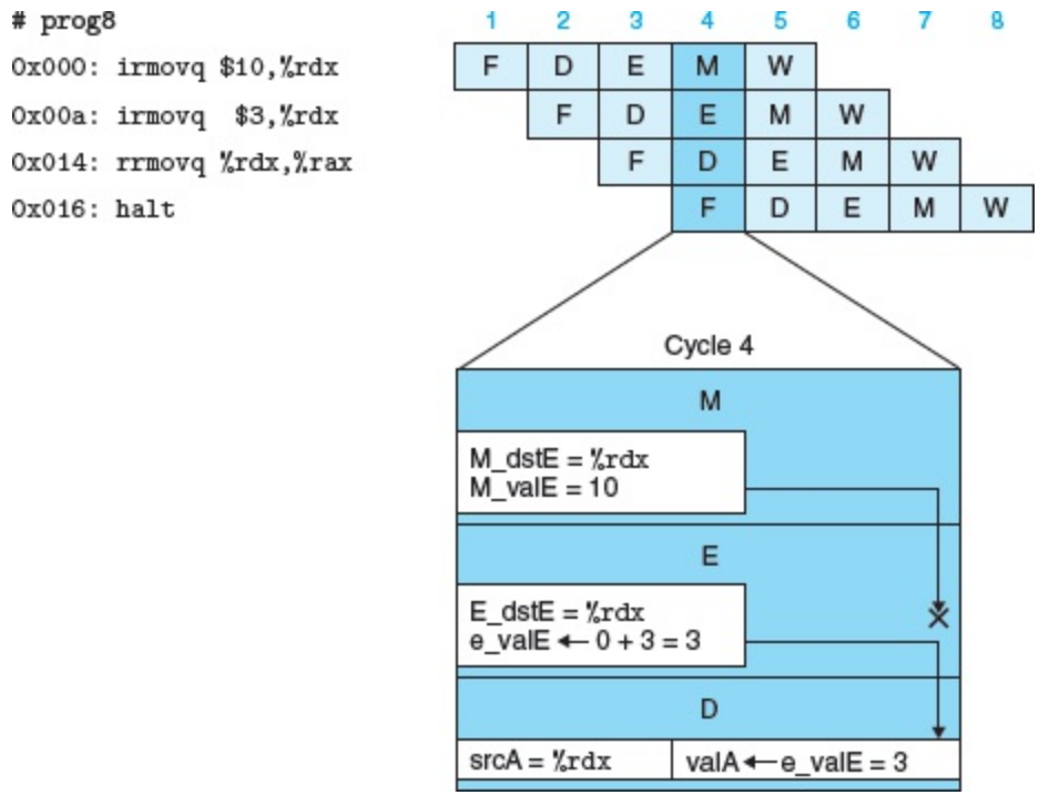
Figure 4.59 Demonstration of forwarding priority.
