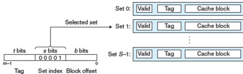
Figure 6.28 Set selection in a direct-mapped cache.
