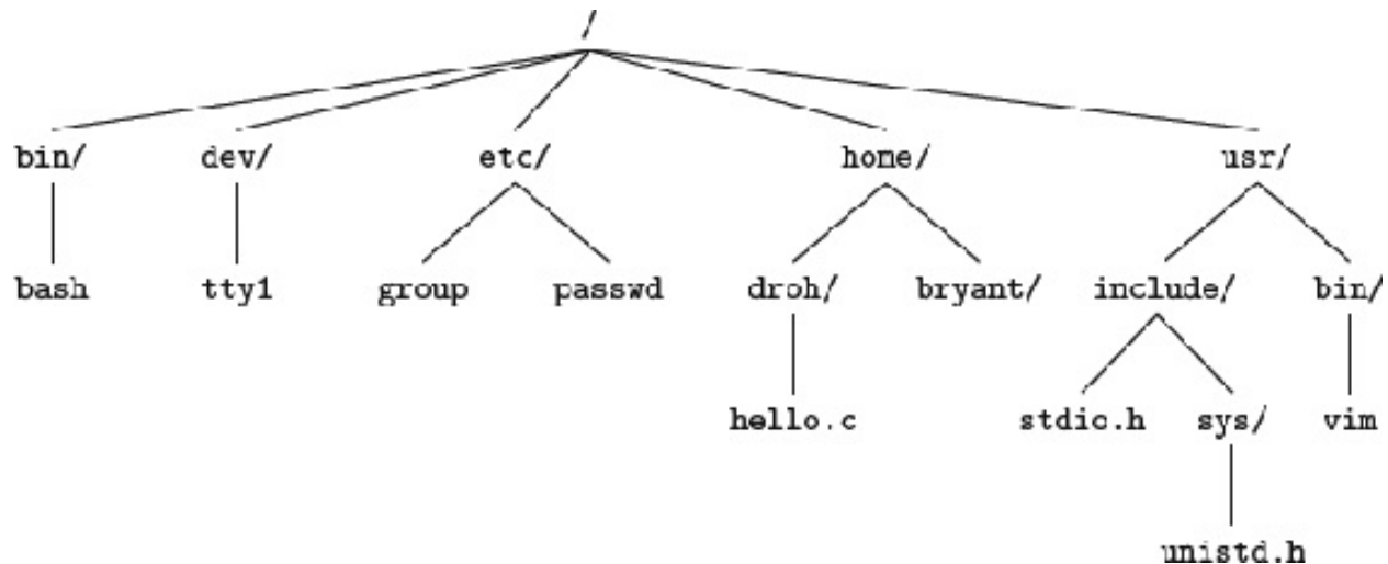
Figure 10.1 Portion of the Linux directory hierarchy.
