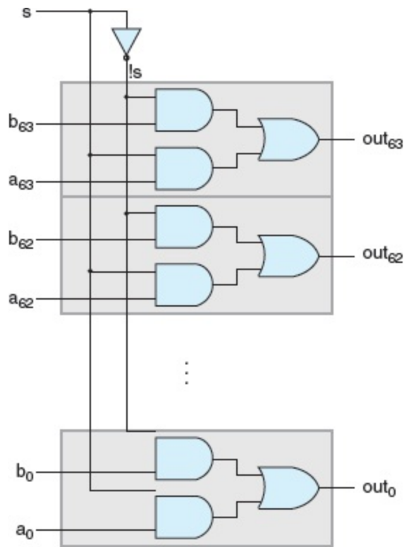
(a) Bit-level implementation
