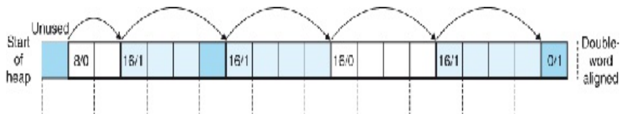
Figure 9.37 Splitting a free block to satisfy a three-word allocation request.
