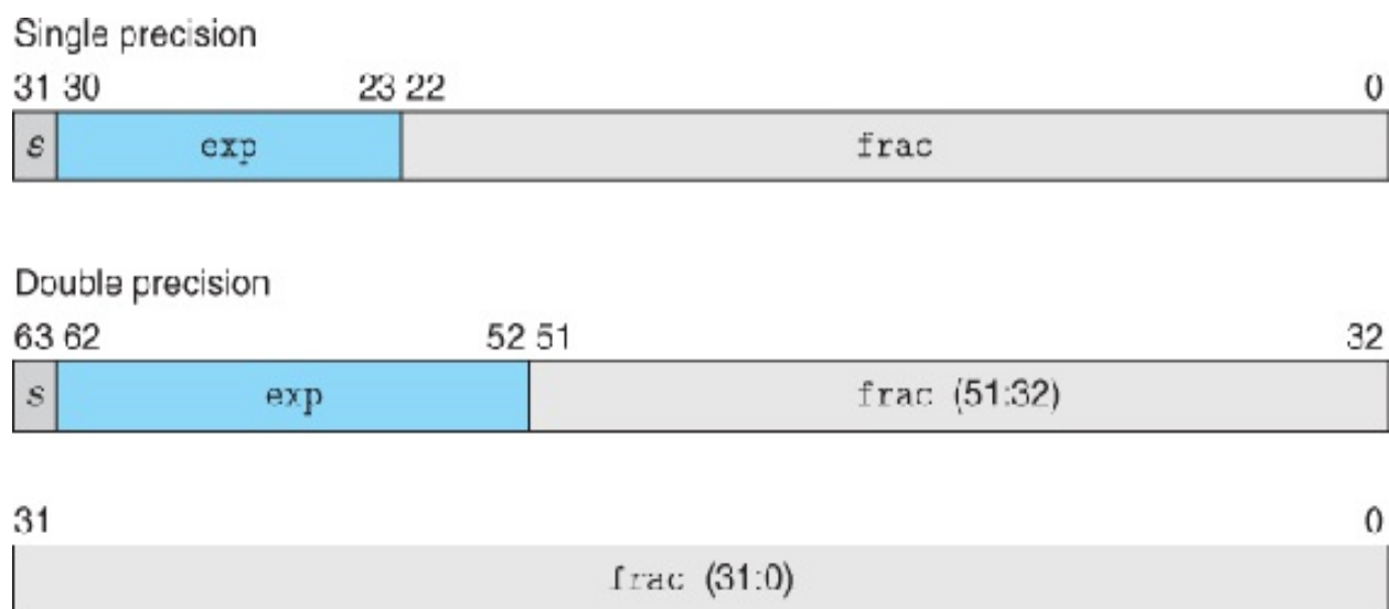
Figure 2.32 Standard floating-point formats.
