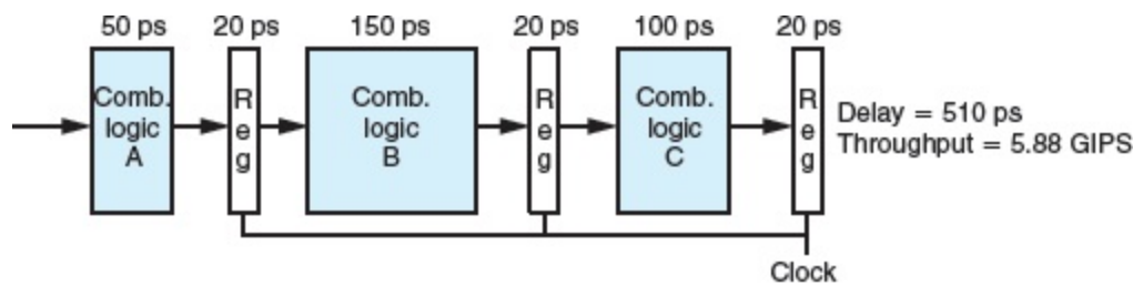
(a) Hardware: Three-stage pipeline, nonuniform stage delays
