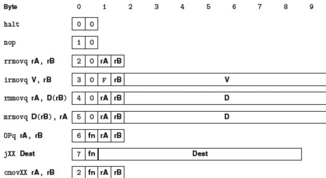
Figure 4.2 Y86-64 instruction set.
